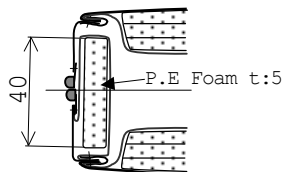
Cross section of side foam.
