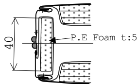
Cross section of side foam.
